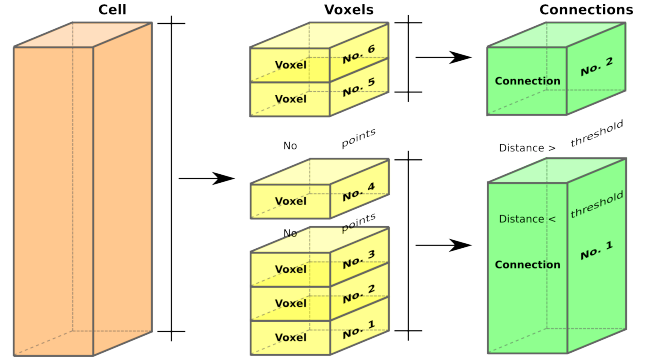
Figure 1: Basic concept: spatial discretization of the ALS point cloud into cell-level (a, left), voxel-level (b, middle) and connection-level (c, right)
