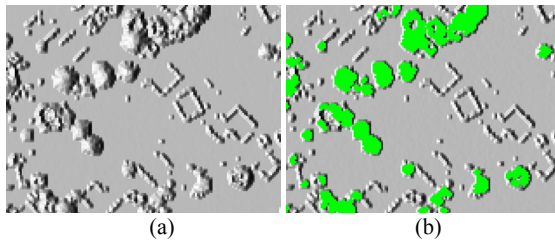
Fig. 3. (a) First-last-echo difference model and (b) the derived enhanced vegetation mask
